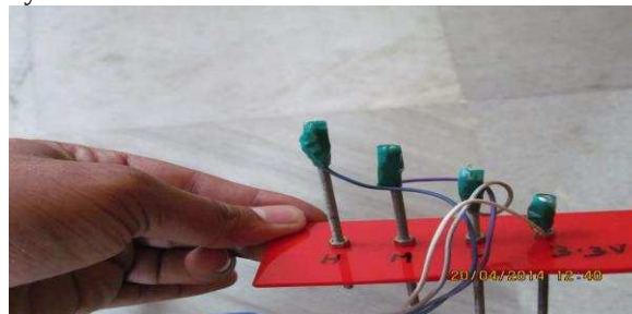
"Fig.17 Water Level Sensor"
